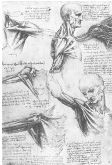
Figure 3. The wire diagram of the human's shoulder by da Vinci 2 (p.15)
