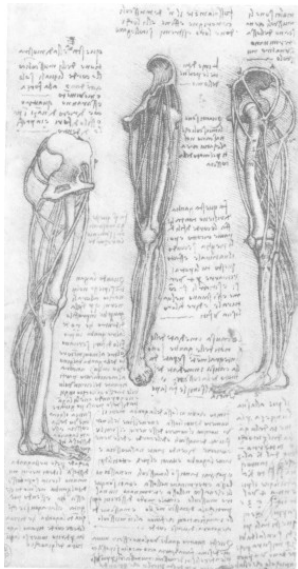
Figure 2. The wire diagram of the human's leg by da Vinci 2 (p.14)
